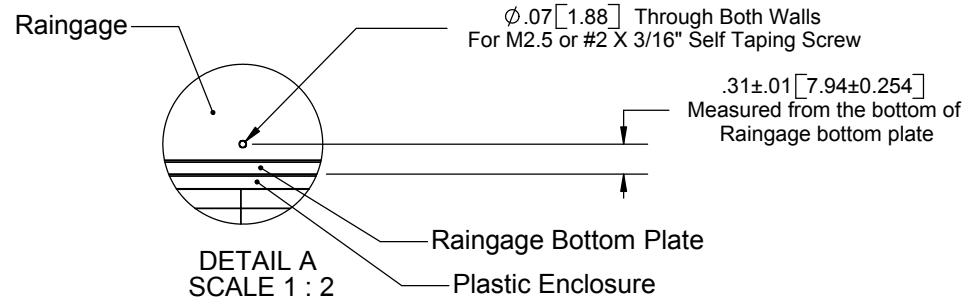
Raingage Retaining Screw (optional)
